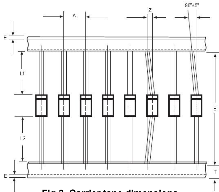
Fig 3. Carrier tape dimensions
